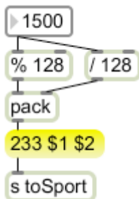
Figure 12. Controlling a servo on pin 9.
