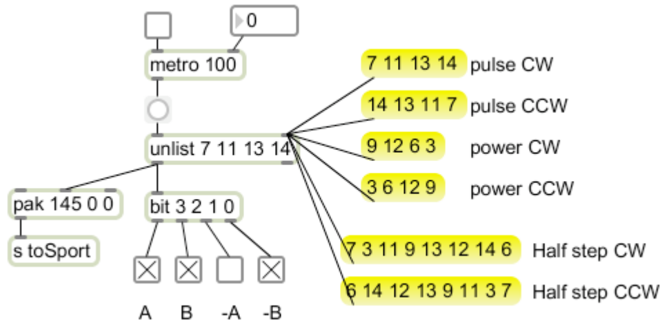
Figure 14. Stepper control
