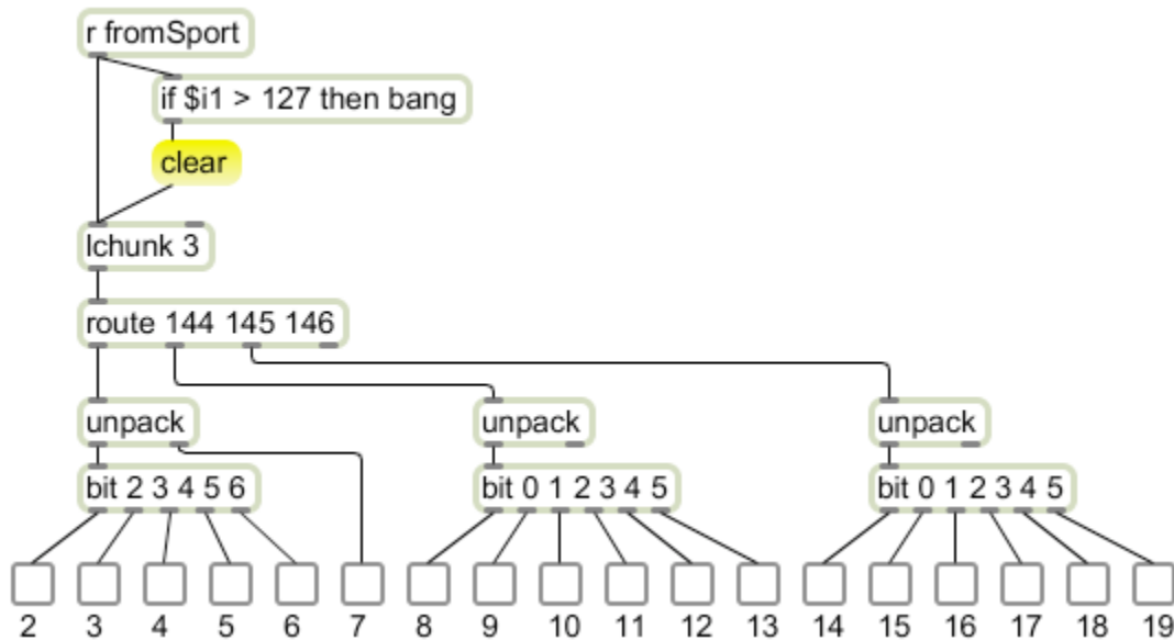
Figure 6. Decoding digital input
