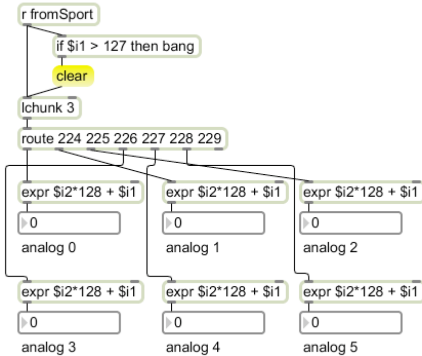
Figure 8. Parsing analog data.
