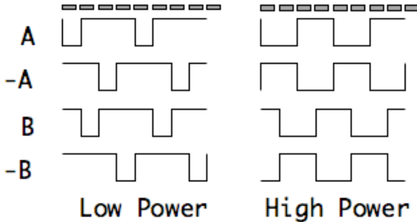
Figure 13. Stepper pulses-- low energizes windings.
